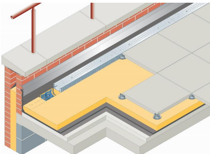
Elevated paver deck
