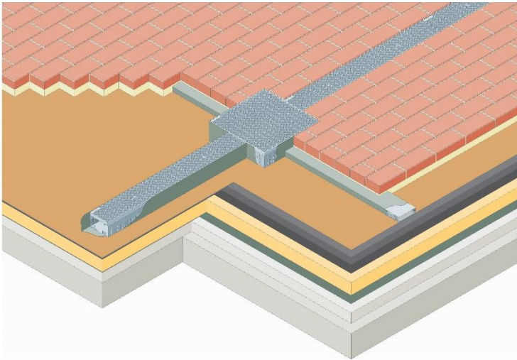
Paved deck on drainage mat
